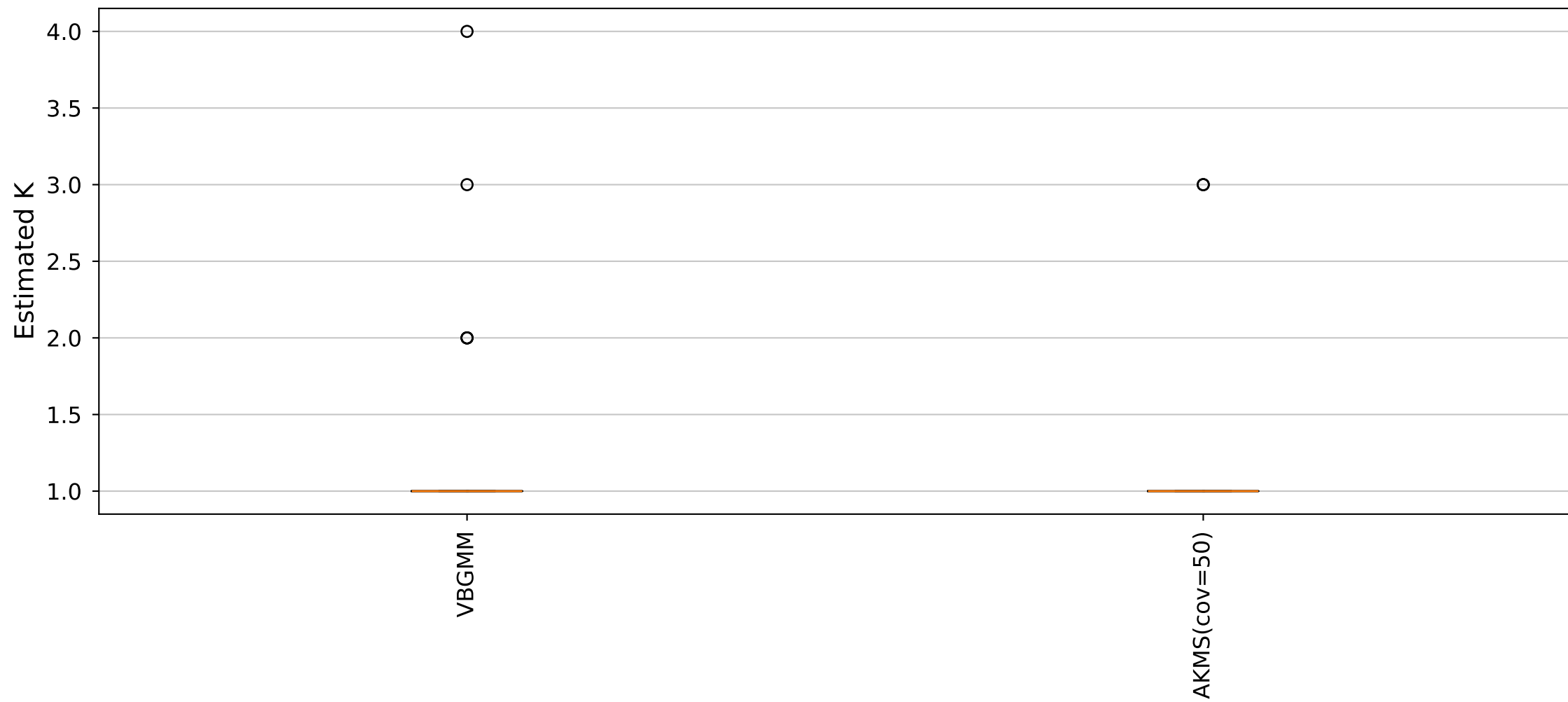
YARA Rules Estimated K Distribution (Cluster5_Size23 dataset)
